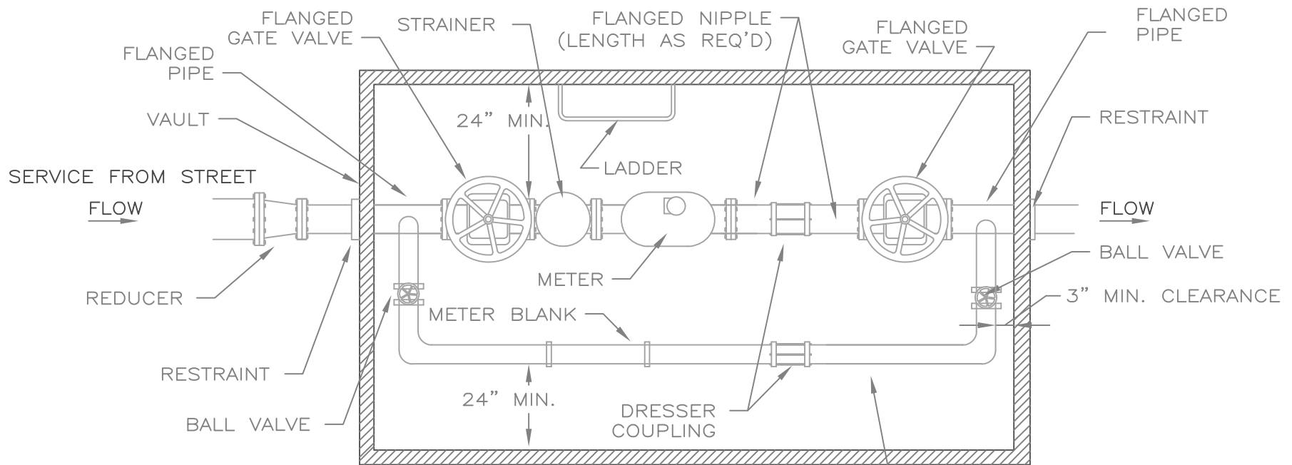
PLAN VIEW
