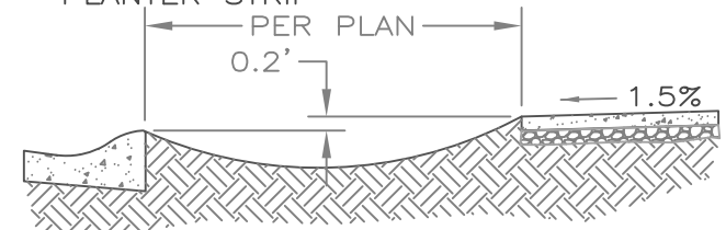
ROLLED CURB
